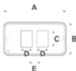
Tampa 2 Módulos RJ11/45 Condulete Top® 1/2" / 3/4"
