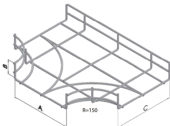
Tê horizontal Horizontal tee Ref. RP 3418
