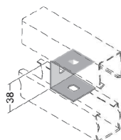
Distanciador "U" quádruplo Fourfold "U" distance piece
