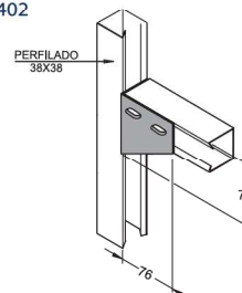
Cantoneira "LR" "LR" angle connector
