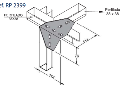
Cantoneira "LR" "LR" angle connector
