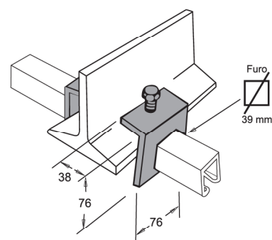
Fixador transversal Transverse support Ref. RP 2405
