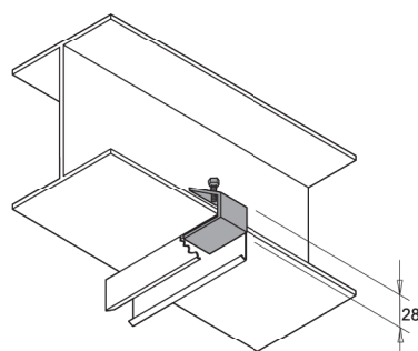
Fixador interno transversal Internal transverse support Ref. RP 2404
