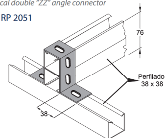
Cantoneira "ZZ" vertical dupla Vertical double "ZZ" angle connector
