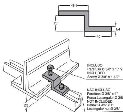
Tala compressora Compressor fishplate Ref. RP 2403
