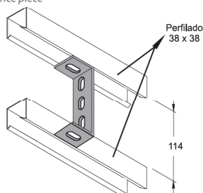
Junção "T" reta Straight "T" plate junction
