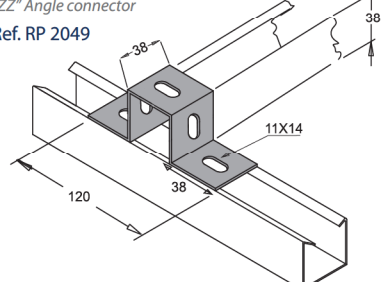
Cantoneira "ZZ" "ZZ" angle connector
