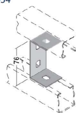
Junção "L" reta Straight "L" plate junction
