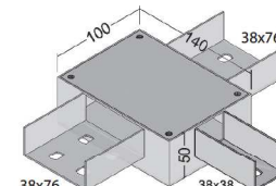
Cx. derivação "C" 38x76 com saída inf. 38x38 "C" Junction box for double channel with one bottom outlet for 38x38 channel
