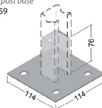
Sapata reforçada Reinforced post base Ref. RP 2057
