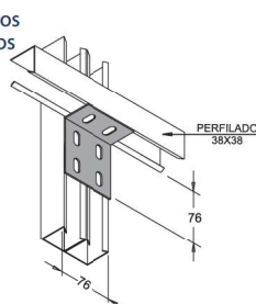
Cantoneira dupla com furos Ten holes doubles angle connector
